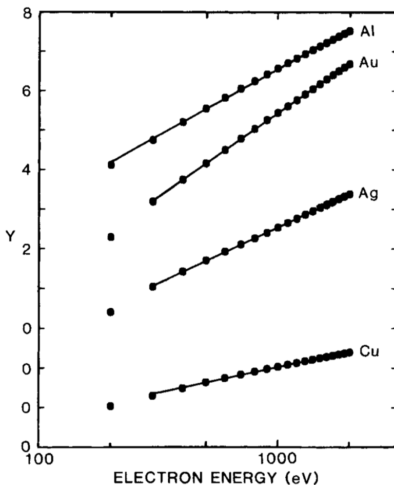
Figure 4. Fano plots for Al, Cu, Ag and Au. From (24), the function Y = 2.12 E \Delta E_a / E_p^2 \lambda_i has been plotted versus electron energy on a logarithmic scale. The plots have been displaced vertically for clarity. The solid circles show values of Y based on the IMFP data in Table 2 and the solid lines show linear least-squares fits.
