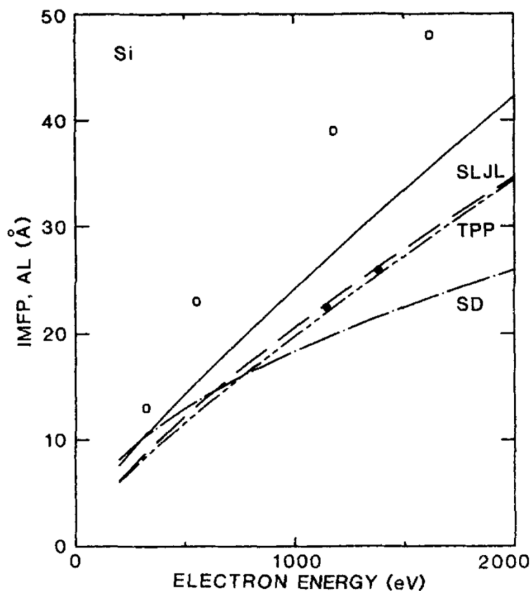
Figure 9. Comparison of IMP and AL results for silicon. The solid line shows IMP values calculated from (1) and (16), as listed in Table 2; the curve devoted TPP is the result of the general formula (24), (27) and (28) using parameter values for Si; the curve designated SLJL is the IMFP result of Szaiman et al. [8] (29a); and the curve denoted SD is the AL result of Seah and Dench,[3] (30). The points show experimental AL values: O, Klasson et al. :[30] ●, overlapping results of Flitsch and Raider[31] and of Ebel and Lieble.[32]
