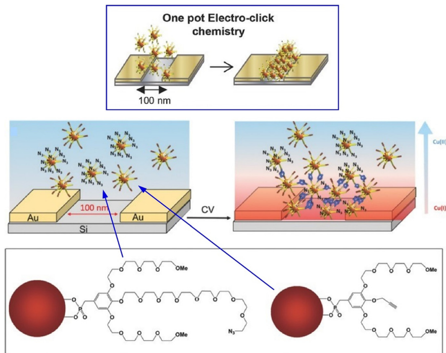
Fig. 17 An electro-click approach for the specific surface integration of gold and iron oxide nanoparticles by covalent bonding into nanodevices to selectively fill the nanotrench. Reprinted with permission from ref. 65 copyright 2015 Wiley-VCH.
