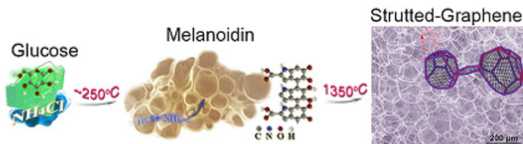
Figure : Scanning electron microscopy images for showing sugar blowing process: glucose were polymerized and blown by released ammonia into melanoidin bubbles in heating, which bubbles were finally converted into strutted graphene containing mono-/few-layered graphene membranes and graphitic struts.
