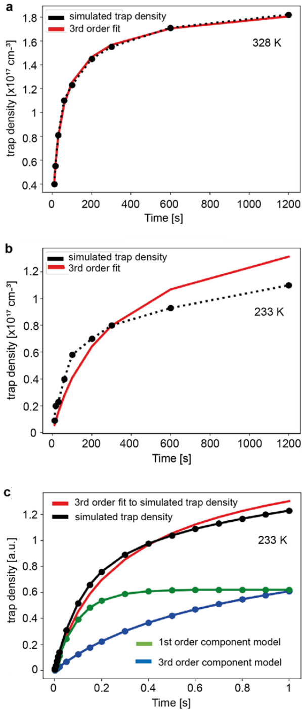
Figure 4. Trap kinetics in electron-only devices. (a) Fit of the simulated trap density at 328 K (data from Figure 1b) to a 3 rd -order kinetics. (b) Fit of the simulated trap density at 233 K (data from Figure 1b) to a 3 rd -order kinetics. (c) Model simulation to demonstrate that the trap density at 233 K can be expressed as a superposition of a slow 3 rd -order kinetic component and a fast 1 st -order component.
