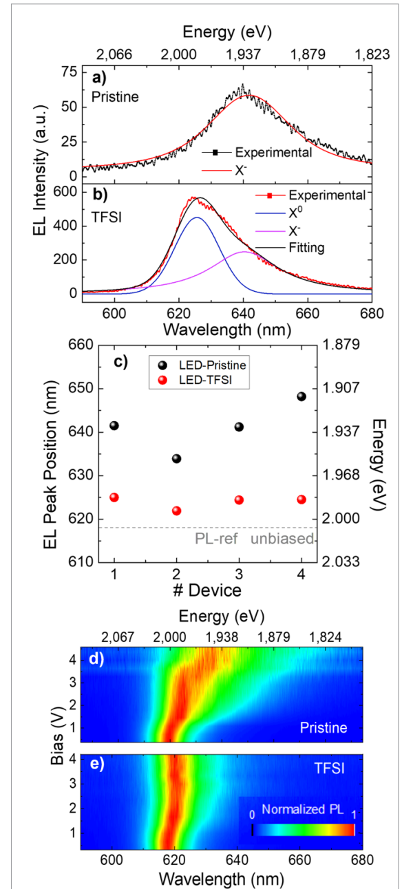
Figure 10. EL spectra of (a) pristine and (b) TFSI-treated LEDs at similar tunneling current \sim 12 \text{ nA} , fitted with Lorentzians. (c) Position of EL emission for different LEDs before (black) and after (red) TFSI. The values in (c) are fits with Lorentzians of EL spectra at similar I , considering the centre of the main emission peak (higher spectral weight). The error bars are within the size of the symbols. Color-plot of the gated-PL of (d) pristine and (e) TFSI-treated LED at similar laser excitation power and integration time.
