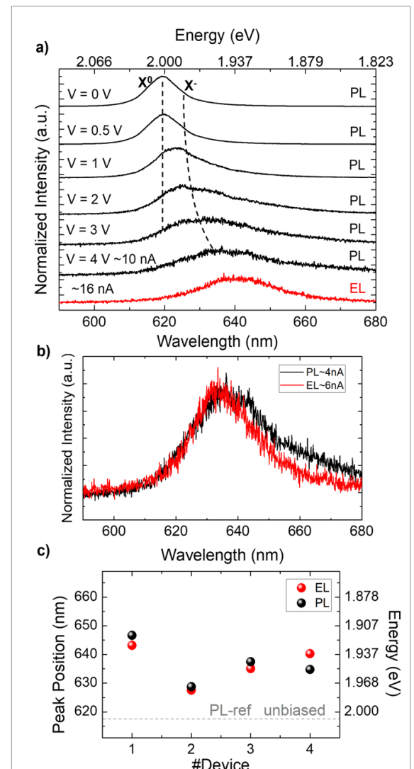
Figure 4. (a) Evolution of PL as a function of V . For comparison, an EL spectrum for I \sim 16 nA is shown (red). The dashed lines are guides to the eye for the X^0 and X^- positions. In all PL measurements up to 3 V, I < 10^{-11} A. At 4 V, I \sim 10 nA, indicating h tunneling through hBN into 1L-WS 2 . (b) Normalized gated-PL and EL spectra of a representative 1L-WS 2 LED near the threshold bias highlighting similarity of the emission spectra. (c) EL and PL positions from 4 different devices. The dashed line plots the unbiased PL position of X^0 measured in figure 3(b). The emission values in (c) are derived by fitting with Lorentzians the PL and EL spectra at similar I level, considering the centre of the main emission peak (higher spectral weight). The error bars are within the size of the symbols.
