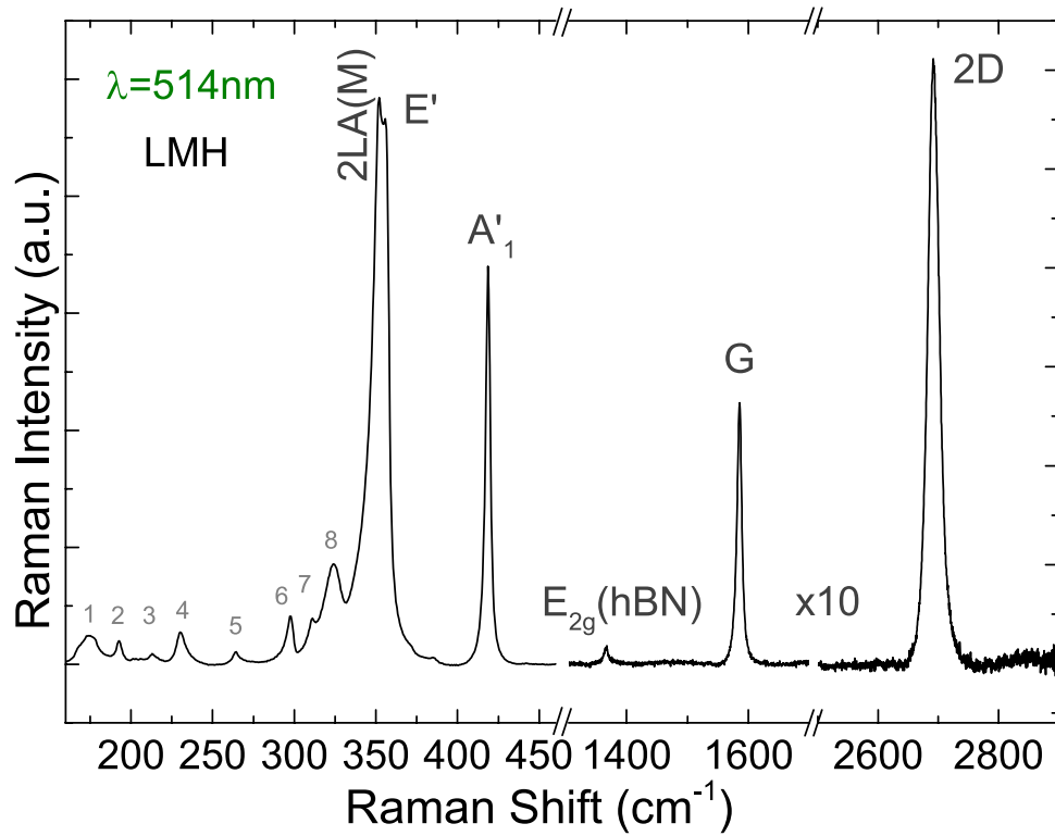
Figure 2. 514.5 nm Raman spectrum of 1L-WS 2 /hBN/SLG LMH after device fabrication. The SLG and hBN Raman modes are labelled. The 1L-WS 2 modes are summarized in table 2. The 1300–2900 cm −1 spectral window is multiplied by a factor 10 for better visualization.
