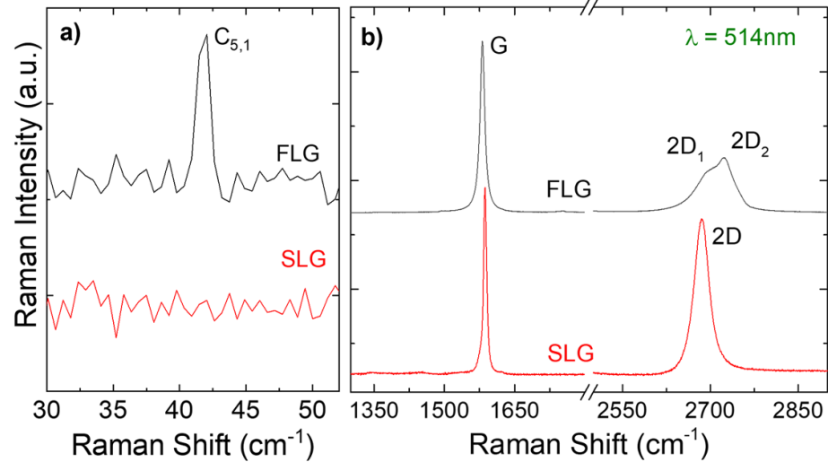
Figure 13. (a) ULF and (b) HF 514.5 nm Raman spectra of SLG and FLG on Si/SiO 2 normalized to the Si peak.
