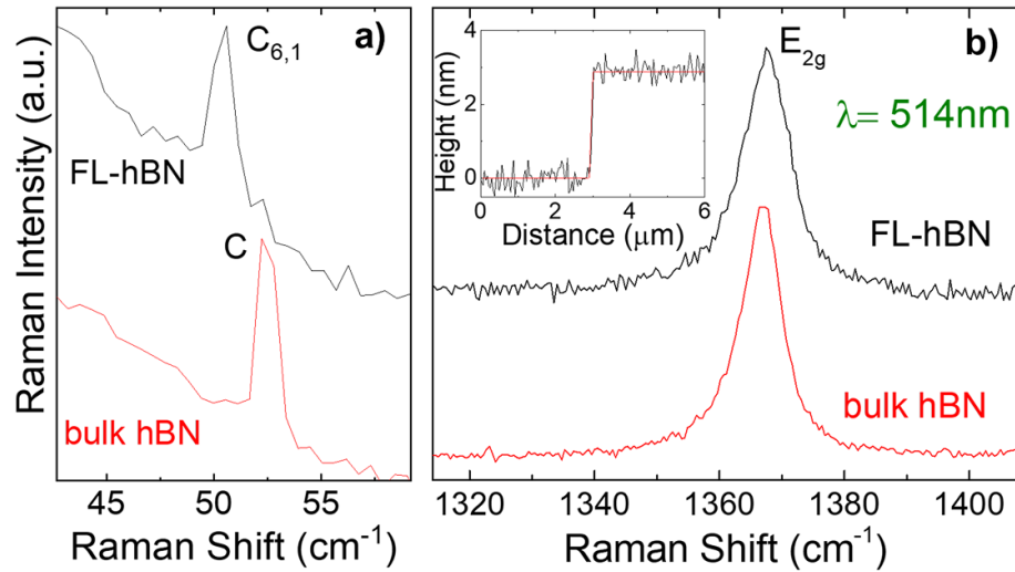
Figure 12. (a) ULF and (b) HF 514.5 nm Raman spectra of \sim 3 nm hBN on Si/SiO 2 normalized to the Si peak. Inset: AFM height profile of \sim 3 nm hBN on Si/SiO 2 .
