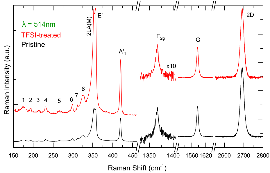
Figure 5. 514.5 nm Raman spectra of pristine (black line) and TFSI-treated (red line) 1L-WS 2 /hBN/SLG. The SLG and hBN Raman modes are labelled, as well as the modes for 1L-WS 2 , as for table 2. The 150–450 cm -1 (1300–2800 cm -1 ) ranges are normalized to the Si (2D) peaks, respectively. The E 2G peak is multiplied by 10 for better visualization.
