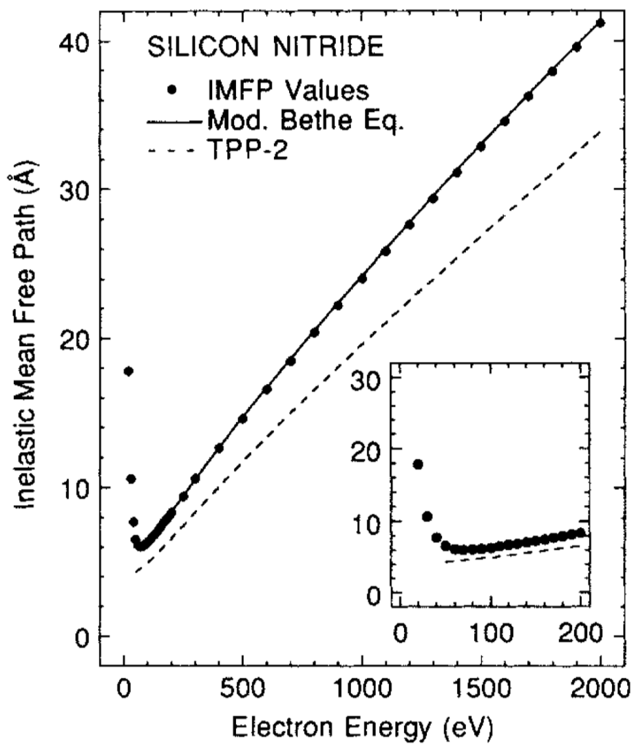
Figure 9. IMFP results for \text{Si}_3\text{N}_4 as a function of electron energy; see caption to Fig. 2.
