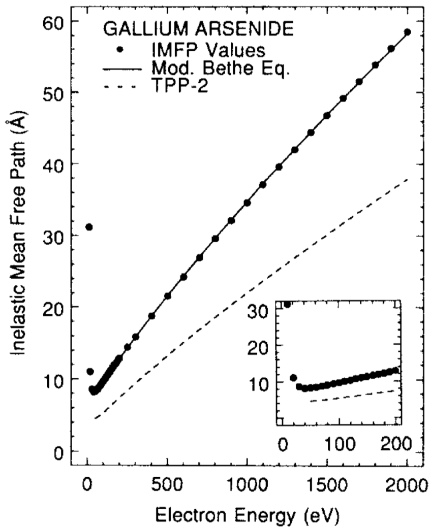
Figure 3. IMFP results for GaAs as a function of electron energy; see caption to Fig. 2.
