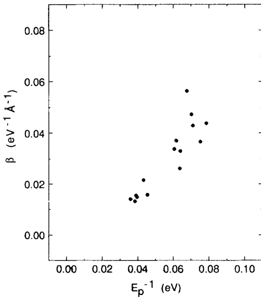
Figure12. Values of \beta found for each compound plotted versus E_p^{-1} (Table 5).
