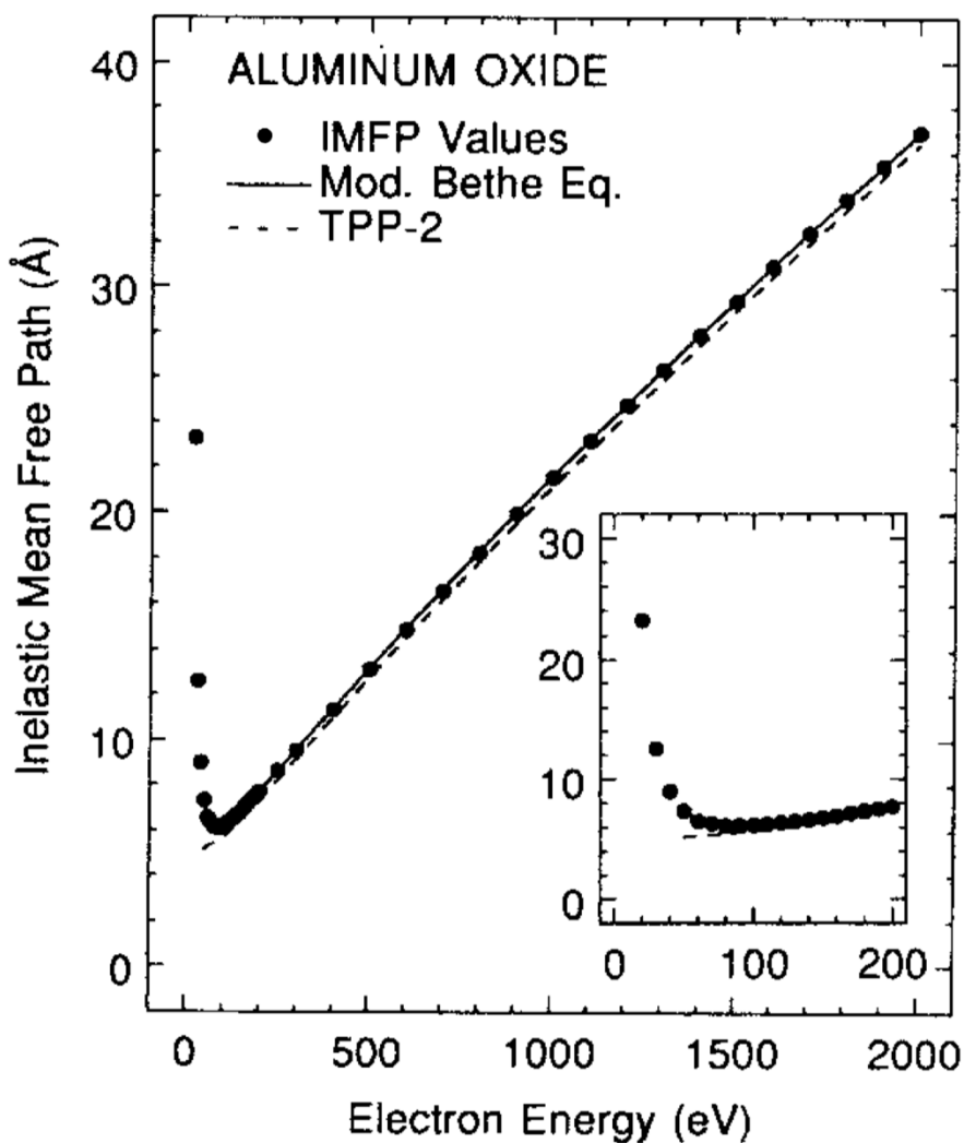
Figure 2. IMFP values (solid circles) calculated for \text{Al}_2\text{O}_3 as a function of electron energy. IMFP values are shown for 10 - 40 eV electrons to illustrate trends but these results are not considered to be reliable (see text). The solid line is a fit to the IMFP values with the modified Bethe equation (Eqn. (4)); values of the parameters found in the fit are given in Table 4. The dashed line shows IMFP values calculated from the predictive formula TPP-2 (Eqn. (4)) where values of the four parameters were calculated from property data for \text{Al}_2\text{O}_3 using Eqn. (5), as indicated in Table 7. The inset shows the low-energy region on an expanded energy scale.
