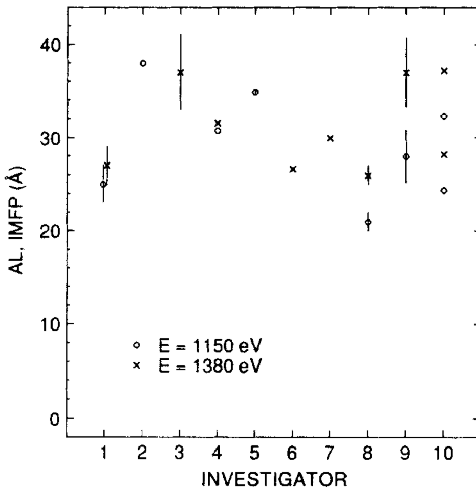
Figure 17. Plot of reported measurements of electron attenuation lengths (ALs) in SiO 2 by nine investigators (Refs 31-39) at two electron energies, 1150 and 1380 eV, corresponding to photoemission of Si L 2,3 -shell electrons by Mg and Al K \alpha x-rays. The values shown as investigator 10 are the IMFP results of this work. Two pairs of IMFP results are shown, one pair (with larger IMFPs) calculated from Eqn. (4) and the parameters of Table 4 and the other pair (with smaller IMFPs) calculated from TPP-2 (Eqns (4) and (5) with parameters listed in Table 7).
