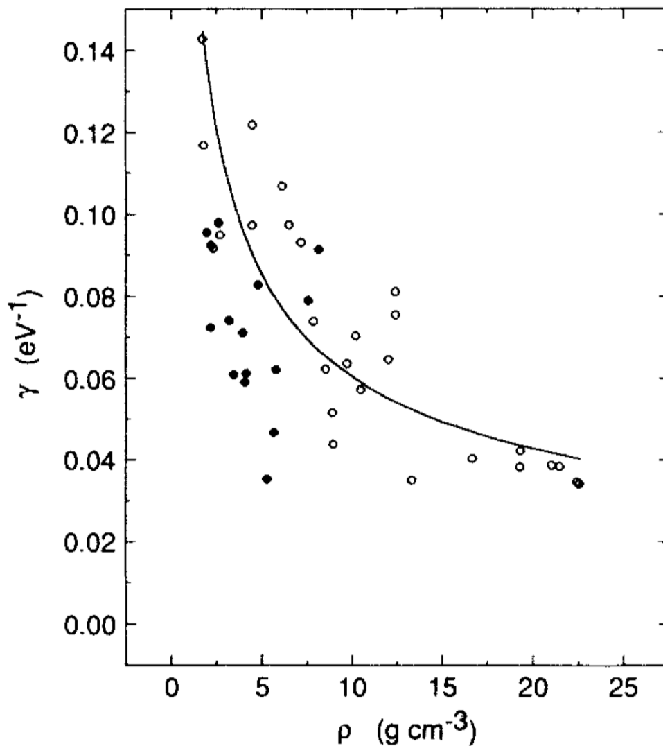
Figure 13. Values of \gamma (solid circles) found for each compound (Table 4) found from the fits of Eqn. (4) to the calculated IMFPs (Table 3) plotted versus density. The open circles show the corresponding results for our group of elements (Ref. 1). The solid line is a plot of Eqn. 5(b).
