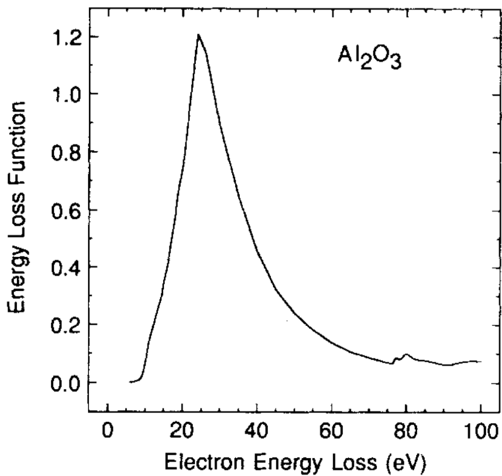
Figure 18. Plot of the electron energy-loss function [\text{Im}(-1/\epsilon(\omega))] for Al 2 O 3 as a function of energy loss \hbar\omega , as calculated from optical data (Table 1).
