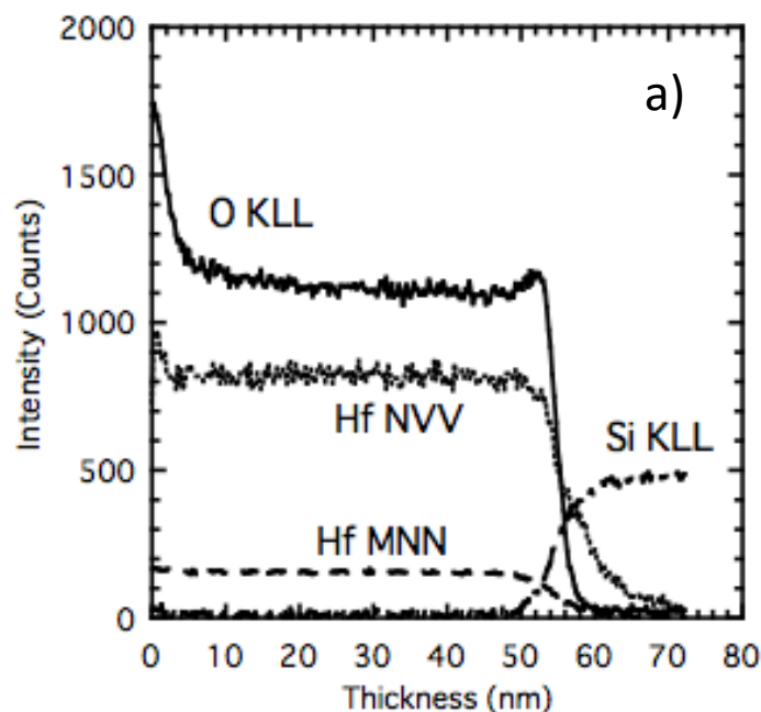
AES depth profiles of the HfO 2 :55 nm/Si substrate using the conventional method with the argon ion energy of 1.0 keV.
