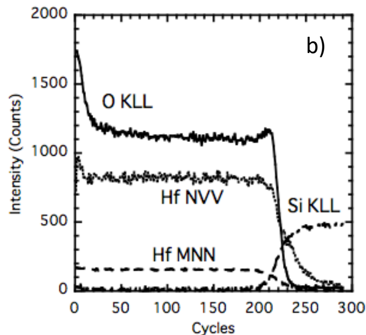
AES depth profiles of the HfO 2 :55 nm/Si substrate using the conventional method with the argon ion energy of 1.0 keV.
