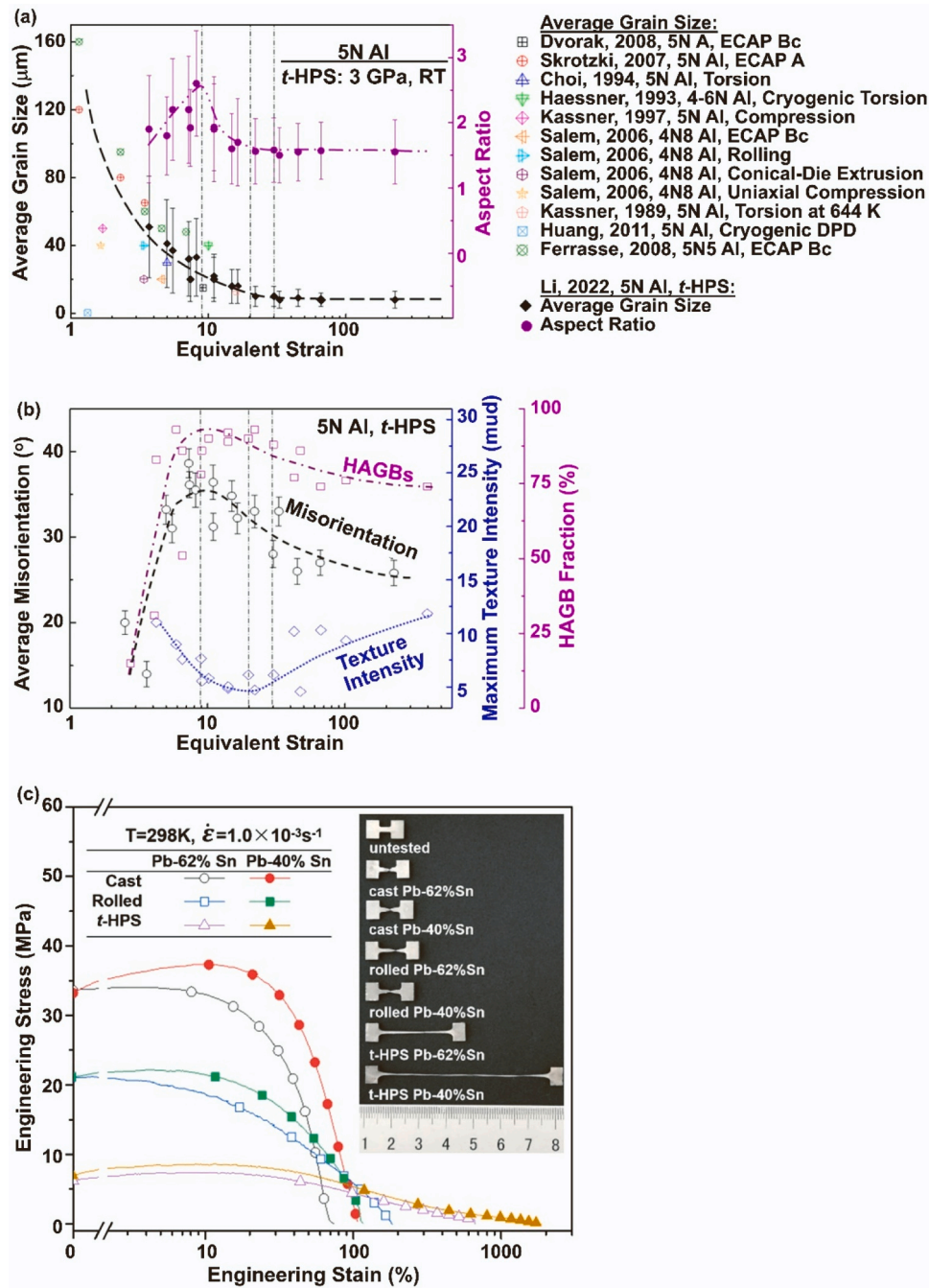
Fig. 9. (a) Evolution of average grain sizes and grain aspect ratios upon increase of t-HPS equivalent strain (grain size obtained from other deformation processing of aluminium with 99.999% purity are also included for comparison) [220]. (b) Evolution of average grain boundary misorientation, high-angle grain boundary fractions and intensity of \{110\}<110> texture upon increase of t-HPS equivalent strain [220]. (c) Engineering stress-strain curves for the Pb-Sn alloys tested at the initial strain rate of 1.0 \times 10^{-3} \text{ s}^{-1} at room temperature (inset: appearance of the specimens after pulling to failure) [201].
