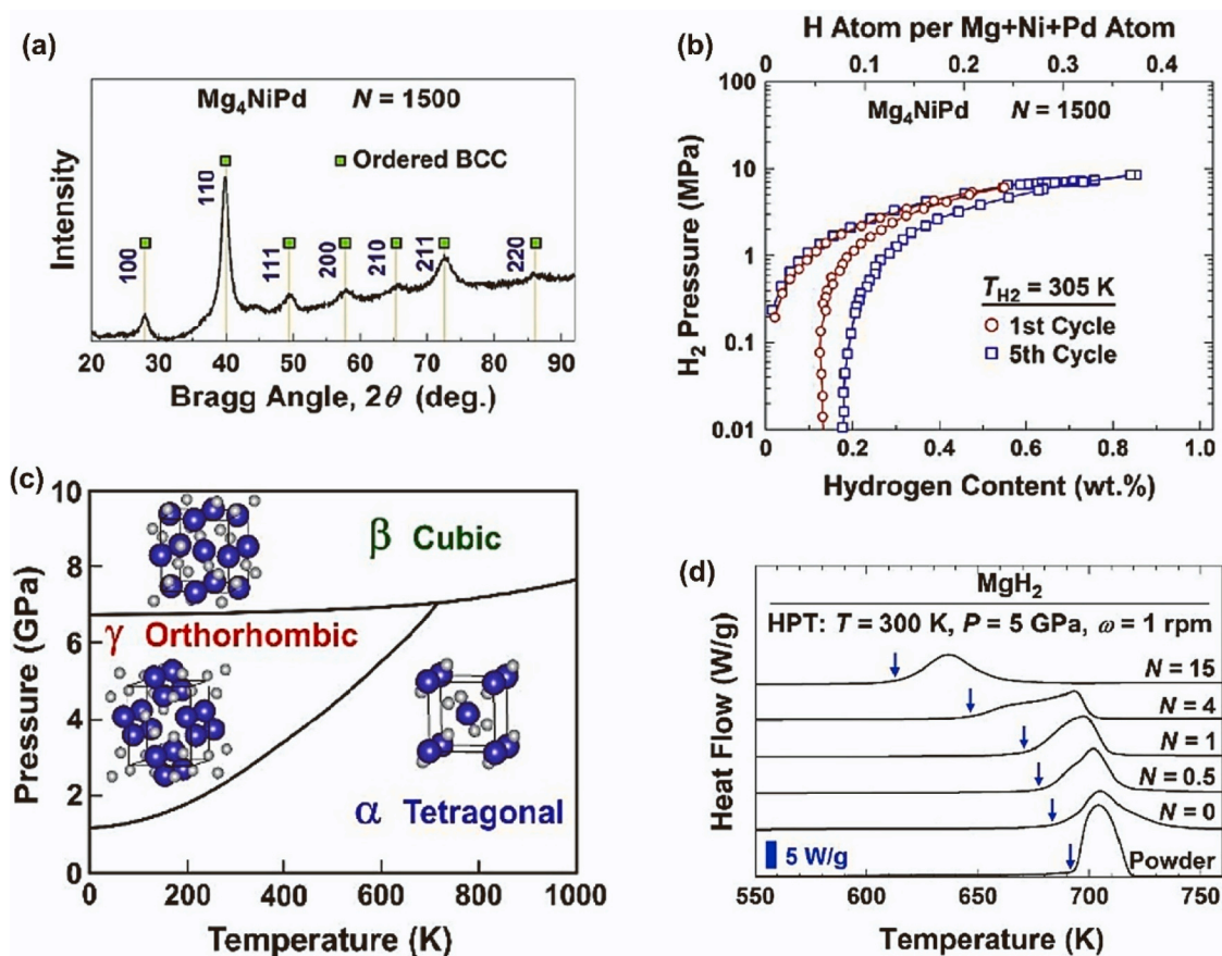
Fig. 53. (a) XRD pattern of Mg 4 NiPd after 1500 HPT turns [359]. (b) Pressure-composition isotherm of Mg 4 NiPd at 305 K [359]. (c) Pressure-temperature phase diagram of MgH 2 [515]. (d) Heat flow in differential scanning calorimetry for MgH 2 processed by HPT for various turns [515].
