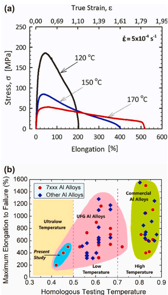
Fig. 68. (a) Deformation curves of a UFG Al-Zn-Mg-Zr (7xxx) alloy, showing a record total elongation higher than 500% at 443 K (homologous temperature: 0.47) [812]. (b) Significance of the UFG structure having grain boundaries segregated by solute atoms, resulting in ultralow-temperature superplasticity in the Al-Zn-Mg-Zr alloy (denoted as Present Study) [812].
