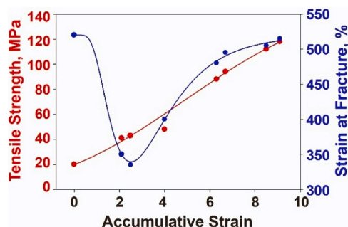
Fig. 89. Influence of the value of accumulated strain on tensile strength and strain at break of high-density polyethylene exposed to ECMAE [1857].
