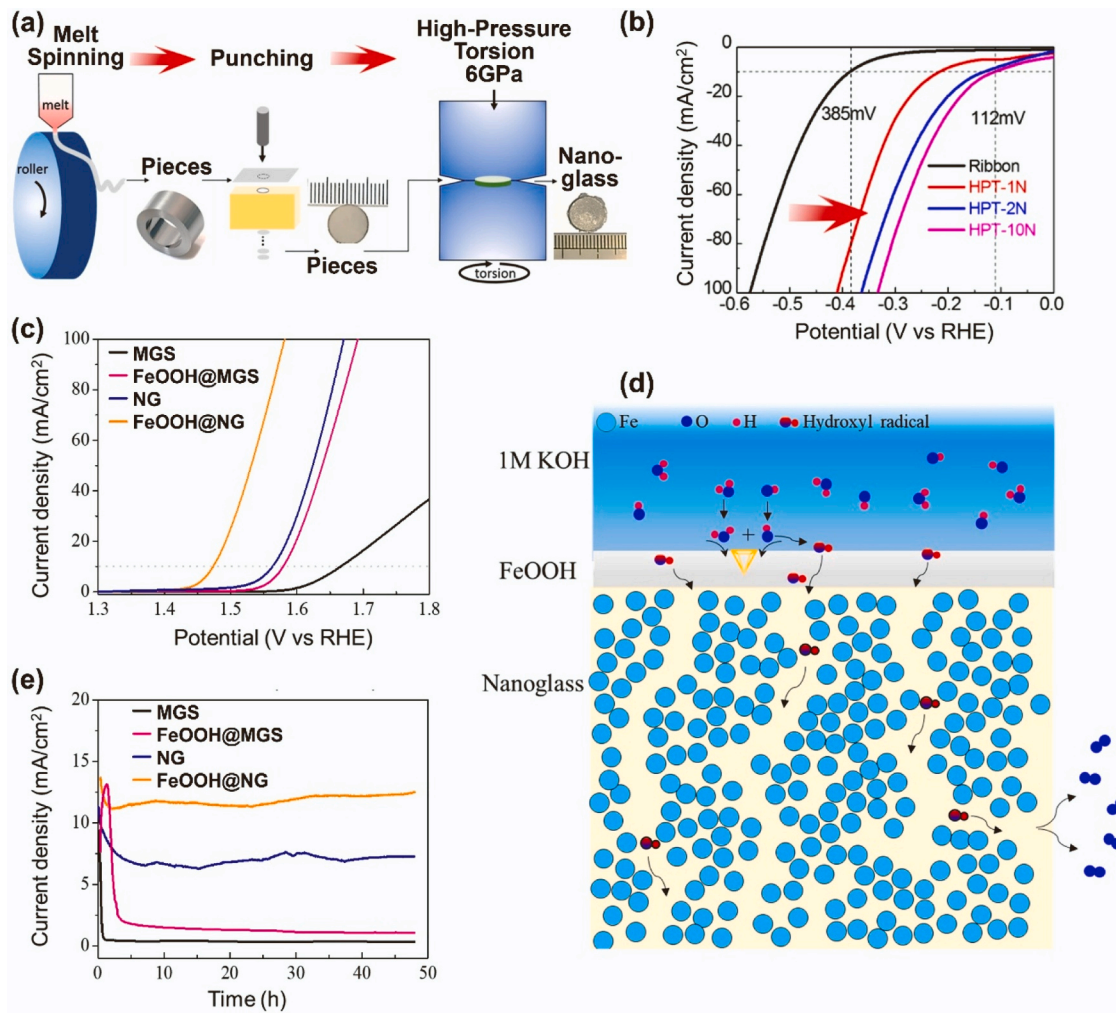
Fig. 49. (a) Schematic illustration for the fabrication of Fe 78 Si 9 B 13 nanoglass alloy [1023]. (b) Linear sweep voltammetry (LSV) curves of the Fe 78 Si 9 B 13 amorphous alloy upon HPT treatment [1023]. (c) LSV curves (iR compensation 90%) of melt-spinning glass (MSG), HPT-processed nanoglass (NG), glass covered by FeOOH (FeOOH@MSG) and nanoglass covered by FeOOH (FeOOH@NG) [1026]. (d) OER catalytic mechanism of the FeOOH@NG [1026]. (e) stability performance obtained from chronoamperometric curves of all samples at the working voltage at 10 mA cm -2 [1026].
