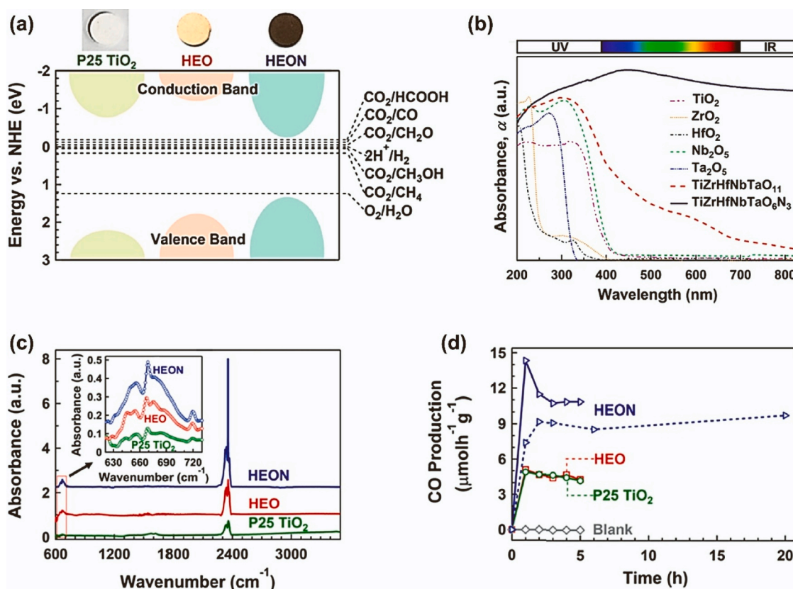
Fig. 47. (a) Electronic band structure of \text{TiZrNbHfTaO}_6\text{N}_3 high-entropy oxynitride (HEON), \text{P25 TiO}_2 and \text{TiZrNbHfTaO}_{11} high-entropy oxide (HEO) [327]. (b) UV-vis light absorbance spectra for \text{TiZrNbHfTaO}_6\text{N}_3 compared to \text{TiZrNbHfTaO}_{11} and corresponding binary oxides [326]. (c) Diffuse reflectance infrared Fourier transform spectra for \text{TiZrNbHfTaO}_6\text{N}_3 compared to \text{P25} and \text{TiZrNbHfTaO}_{11} [327]. (d) Rate of \text{CO} production for \text{TiZrNbHfTaO}_6\text{N}_3 compared to \text{P25 TiO}_2 and \text{TiZrNbHfTaO}_{11} [327].
