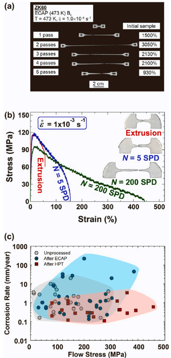
Fig. 66. (a) Appearance of tensile specimens of a ZK60 alloy processed by different number of passes of ECAP and tested at 473 K [1475]. (b) Stress vs. strain curves and appearance of tensile specimens of an Mg-8Li (wt%) alloy processed by extrusion and different number of turns of HPT and tested at room temperature [350]. (c) The corrosion rate of magnesium and magnesium alloys plotted as a function of the flow stress [1478].
