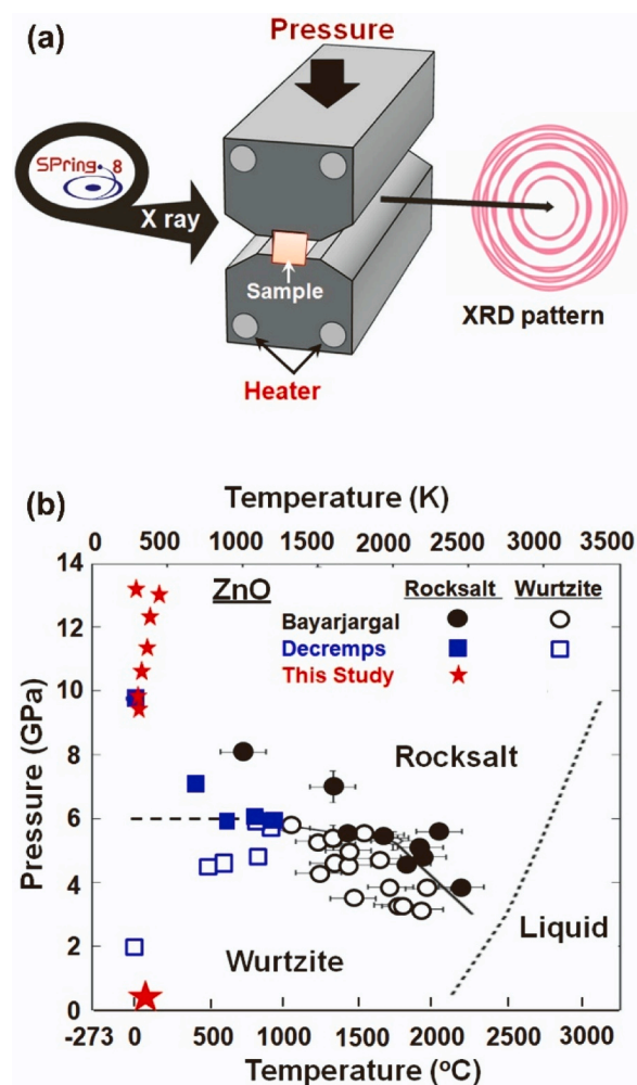
Fig. 28. (a) Schematic illustration of high-pressure application system for in situ XRD analysis at SPring-8, Japan [607]. (b) Temperature-pressure phase diagram of \text{ZnO} . Open and closed circles are reproduced from Bayarjargal and Winkler [593] for wurtzite and rocksalt structures, respectively. Open and closed blue squares are from Decremps et al. [594], representing transformation points from rocksalt to wurtzite structure and from wurtzite to rocksalt structure, respectively. Star symbols represent results of HPT-processed \text{ZnO} in which rocksalt occupies 100% [607].
