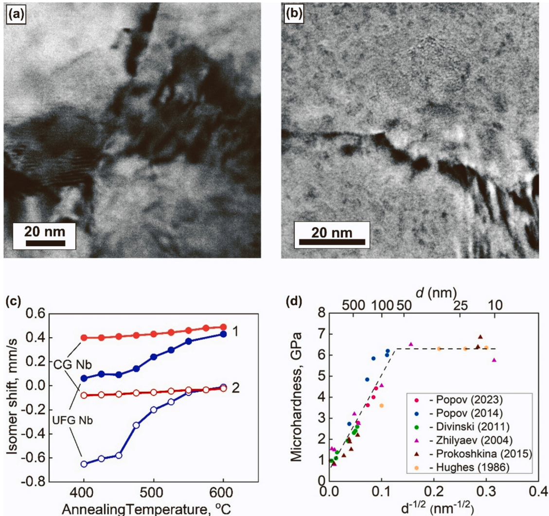
Fig. 19. (a,b) Stepwise boundaries in HPT-processed (a) niobium and (b) nickel [407]. (c) Isomer shifts of ^{57}\text{Co}(^{57}\text{Fe}) spectral lines versus annealing temperature in coarse-grained niobium (red lines and symbols) and UFG niobium (blue lines and symbols) [406]. (d) Microhardness versus grain size ( d ) in nickel processed by various techniques [407].
