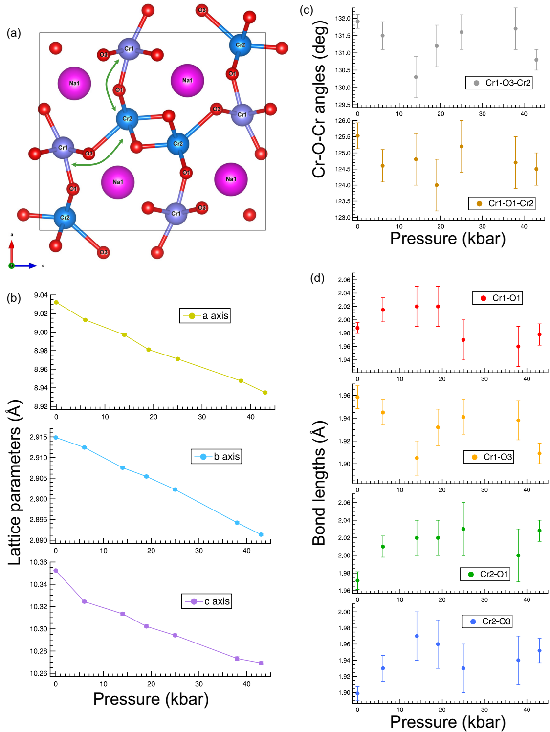
FIG. 10. (a) Schematic of NaCr 2 O 4 crystal structure with the Cr1/Cr2 and O1/O3 sites explicitly labeled and the Cr–O–Cr bonds of interest highlighted by green arrows. (b) Pressure-dependent trends of the lattice parameters a , b and c , the straight line is a guide to the eye. (c) Pressure-dependent trends of the Cr1–O3–Cr2 and Cr1–O1–Cr2 angles. (d) Pressure-dependent trends of the short Cr–O bond lengths.
