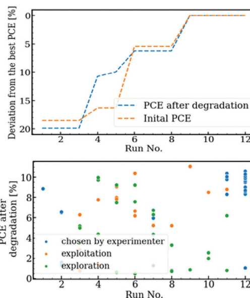
Figure 7. Example of an autonomous optimization of a quaternary OPV-mixture performed on AMANDA/Line1. The Bayesian optimizer Phoenix was used to optimize two objectives (initial efficiency and efficiency after aging test) in a 3D-process parameter space. Six samples were investigated in each iteration, the optimum was found after nine iterations. (Reproduced with permission. [53] Copyright 2021, Tobias Osterrieder.).
