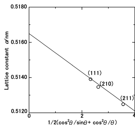
Fig. 5 Lattice constant as function of the diffraction degree, \theta , for the solid-state cubic ammonia ( \text{NH}_3(\text{cr}) ) at 297 K.
