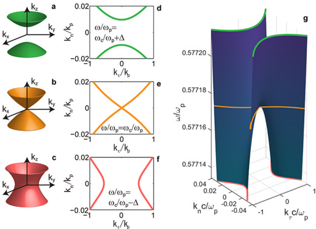
Figure 1: a-f , Iso-frequency curves of the multilayer HMM in k_x - k_y - k_z space ( a-c ) and in k_t - k_n space ( d-f ) at \omega/\omega_p = \omega_c/\omega_p + \Delta ( a, d ), \omega/\omega_p = \omega_c/\omega_p ( b, e ) and \omega/\omega_p = \omega_c/\omega_p - \Delta ( c, f ). Panel ( g ) shows the evolution of iso-frequency curve with frequency, in the range \omega_c/\omega_p - \Delta \leq \omega/\omega_p \leq \omega_c/\omega_p + \Delta . The iso-frequency curves in panels d-f are superimposed in panel g with the same colors. Throughout the entire plot, c is the speed of light, \omega_p is the plasma frequency of the metal layer consisting HMM, k_p = \omega_p/c and \Delta = 2.5 \times 10^{-5} .
