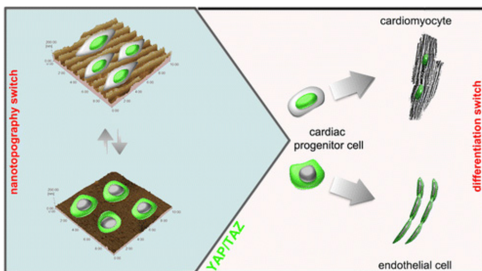
Figure : Schematic illustrating how mechanical properties of substrates affect where YAP/TAZ protein localization in cardiac stem cells (left) and how this affects stem cell development and function (right).
